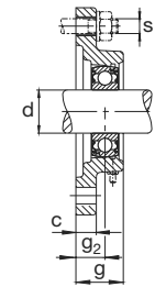
FL762..2RSR
