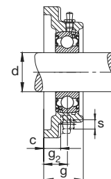
F762..2RSR
