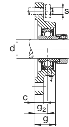
FL362
