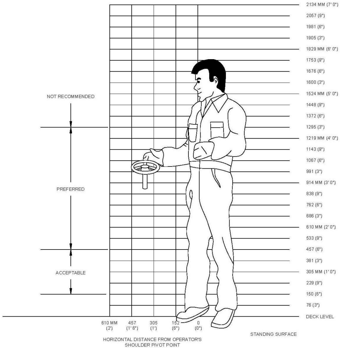
FIGURE 87. Mounting heights for handwheel valves with vertical stems.
