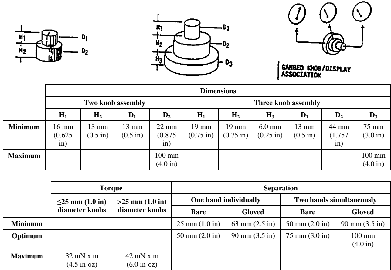
FIGURE 11. Ganged knobs.
