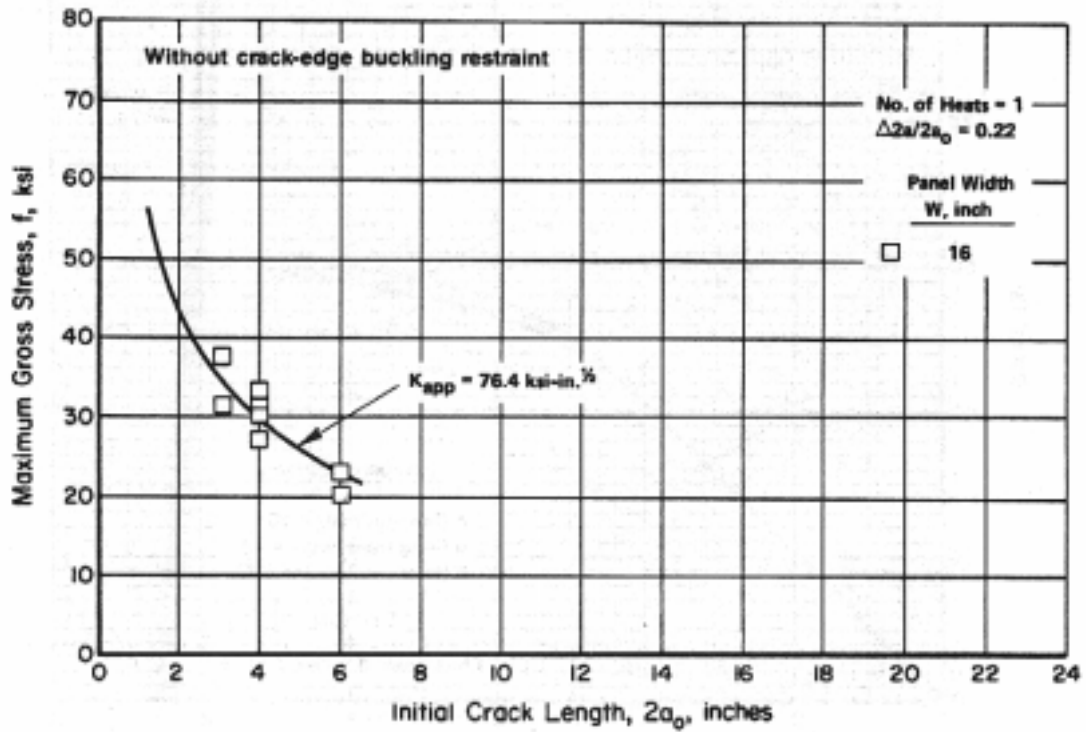
Figure 3.7.8.10(c). Residual strength behavior of 0.063-inch-thick 7475-T61 clad aluminum alloy sheet at room temperature. Crack orientation is L-T. [Reference 3.2.5.1.9(d).]
