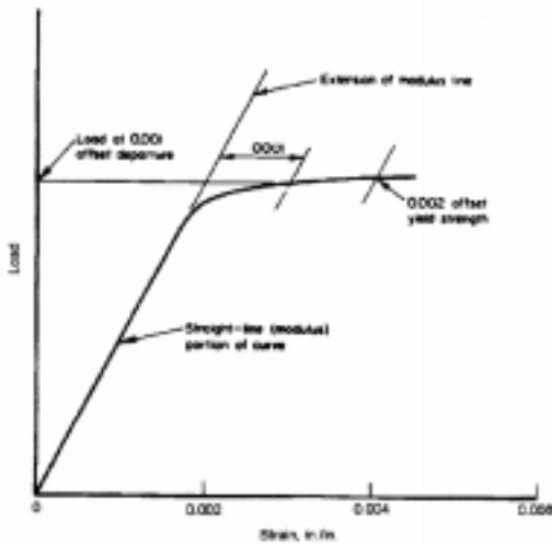
Figure 9.3.2.3(a). Measuring loads by strain departure method.
