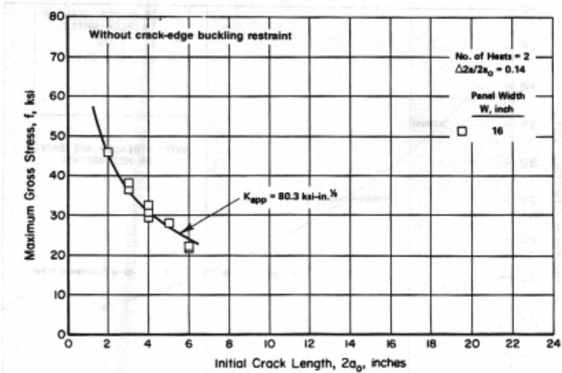
Figure 3.7.8.1.10(a). Residual strength behavior of 0.063-inch-thick 7475-T61 aluminum alloy sheet at room temperature. Crack orientation is L-T. [References 3.1.2.1.6(d) and 3.2.5.1.9(d).]
