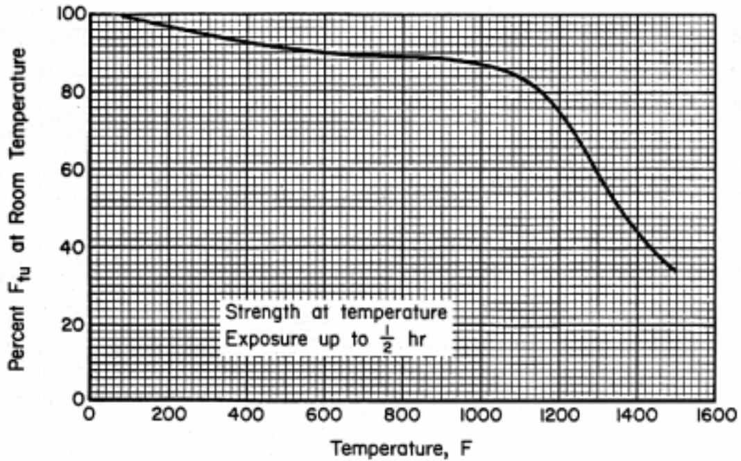
Figure 6.3.6.2.1(a). Effect of temperature on the tensile ultimate strength ( F_{tu} ) of Inconel X-750 bar (AMS 5667).
