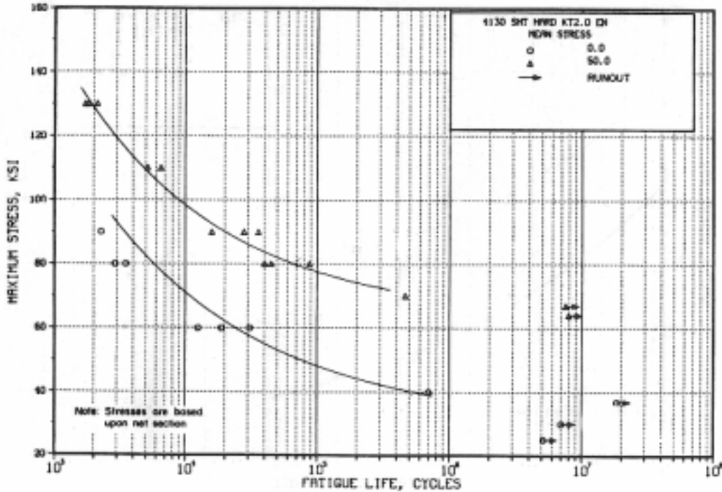
Figure 2.3.1.2.8(g). Best-fit S/N curves for notched, K_t = 2.0 , 4130 alloy steel sheet, F_u = 180 ksi, longitudinal direction.
