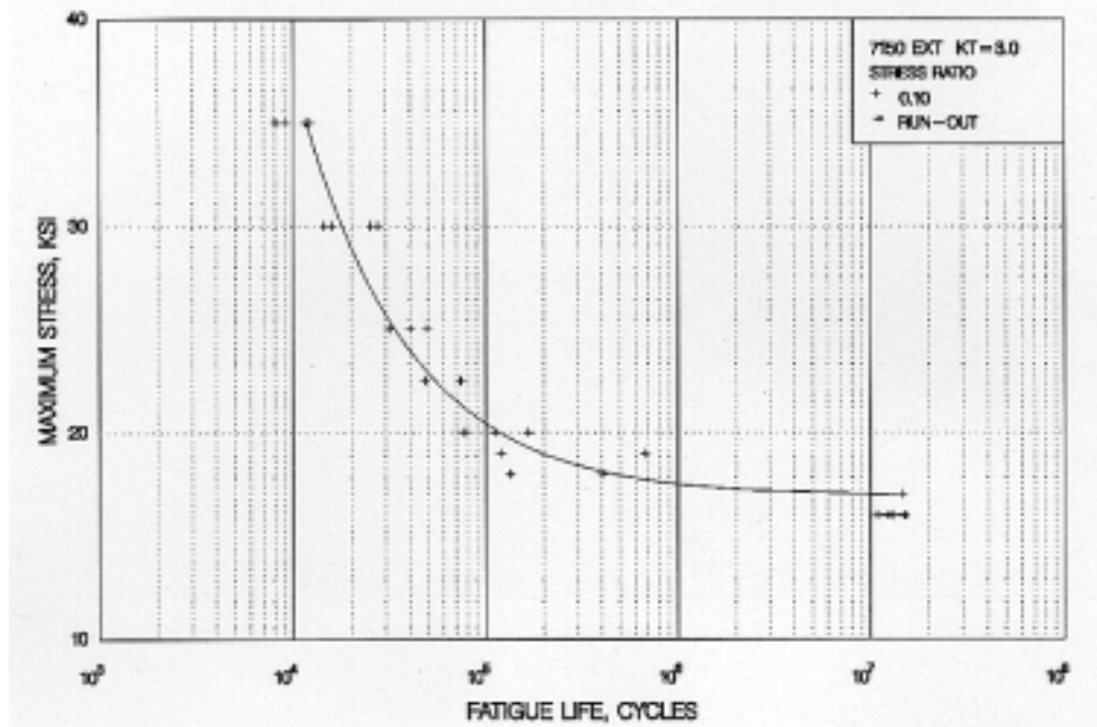
Figure 3.7.5.2.8(c). Best-fit S/N curves for notched, K_t = 3.0 , 7150-T7751 aluminum alloy extrusion, longitudinal and long transverse orientations.
