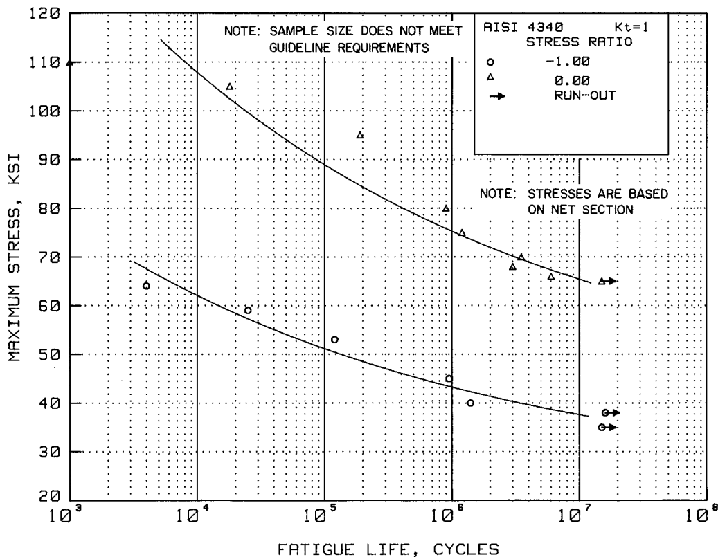
Figure 2.3.1.3.8(i). Best-fit S/N curves for unnotched AISI 4340 alloy steel bar at 1000°F, F_{10} = 150 ksi, longitudinal direction.
