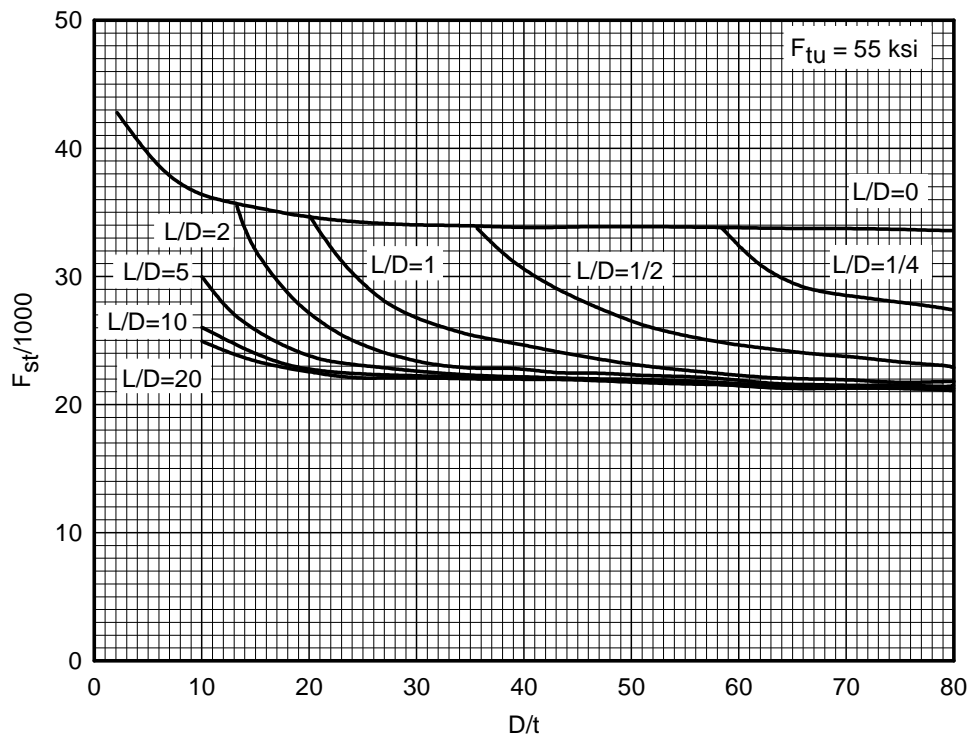
Figure 2.8.3.2(a). Torsional modulus of rupture—plain carbon steels F_{tu} = 55 ksi.
