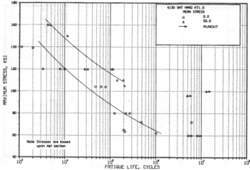
Figure 2.3.1.2.8(f). Best-fit S/N curves for unnotched 4130 alloy steel sheet, F_{1u} = 180 ksi, longitudinal direction.
