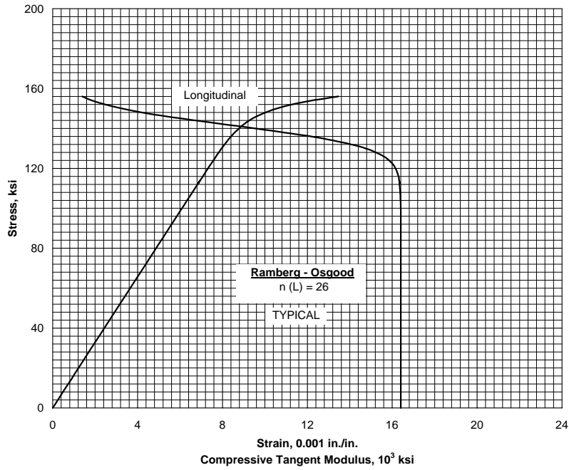
Figure 5.5.2.1.6(a). Typical tensile stress-strain curves at room temperature for solution treated and aged ( 1000^\circ\text{F} ) Ti-15V-3Cr-3Sn-3Al alloy sheet.
