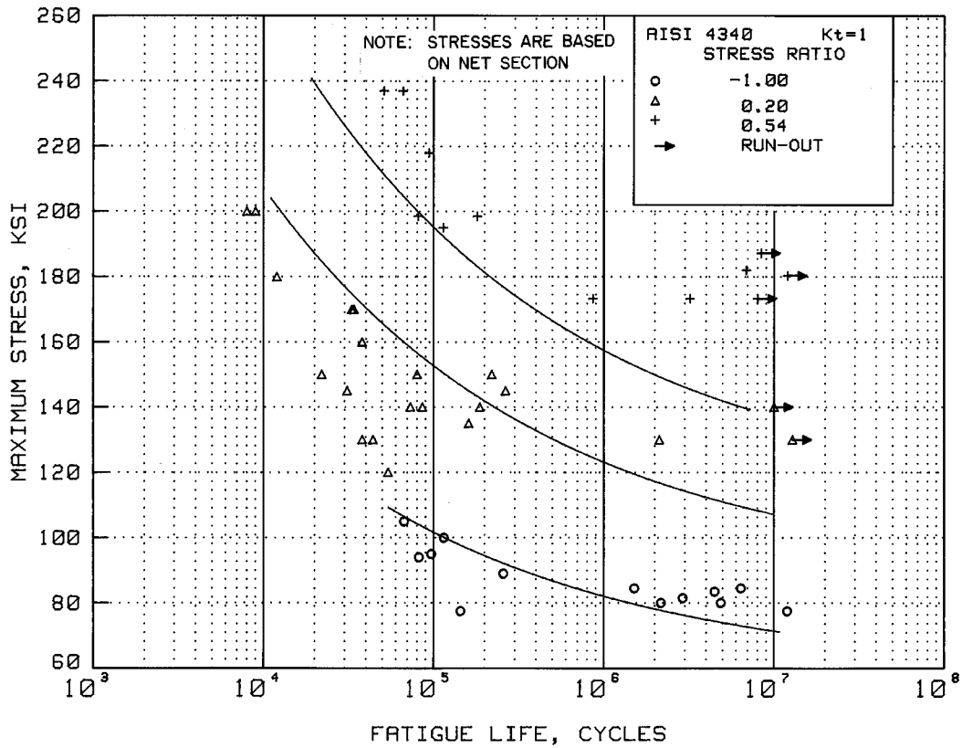
Figure 2.3.1.3.8(m). Best-fit S/N curves for unnotched AISI 4340 alloy steel bar and billet, F_u = 260 ksi, longitudinal direction.
