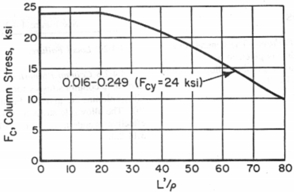
Figure 4.4.2.3(b). Allowable column stresses for AZ31B-H24 magnesium-alloy sheet.
