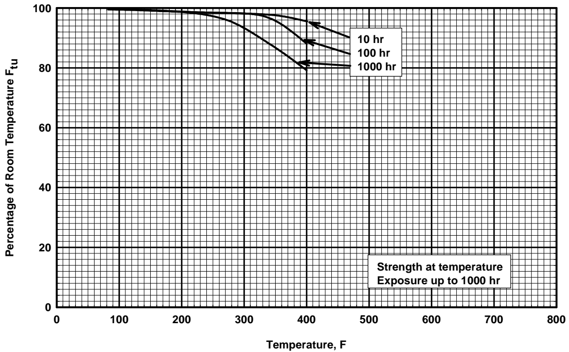
Figure 3.2.10.1.1(d). Effect of exposure at elevated temperatures on room-temperature tensile ultimate strength ( F_{tu} ) of 2618-T61 hand forging.
