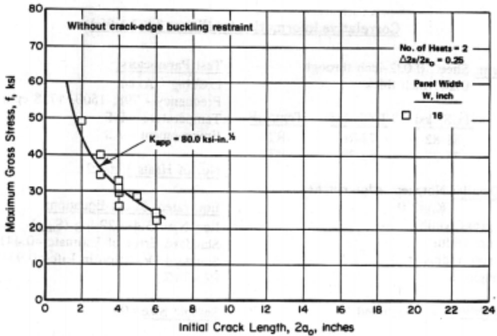
Figure 3.7.8.1.10(b). Residual strength behavior of 0.063-inch-thick 7475-T61 aluminum alloy sheet at room temperature. Crack orientation is T-L. [References 3.1.2.1.6(d) and 3.2.5.1.9(d).]
