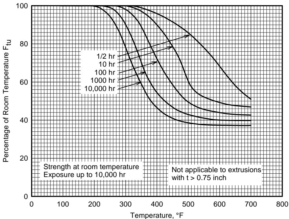
Figure 3.2.1.1.1(e). Effect of exposure at elevated temperatures on the room-temperature tensile ultimate strength ( F_{tu} ) of 2014-T6, T651, T6510, and T6511 aluminum alloy (all products except thick extrusions).
