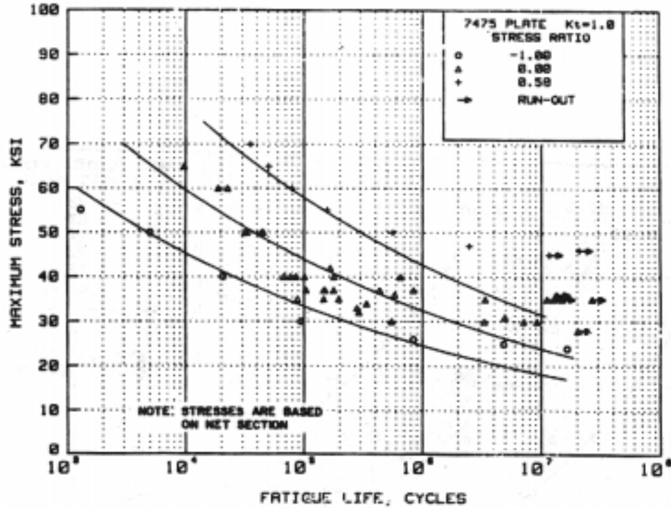
Figure 3.7.8.2.8(a). Best-fit S/N curves for unnotched 7475-T7351 plate, longitudinal and long transverse orientation.
