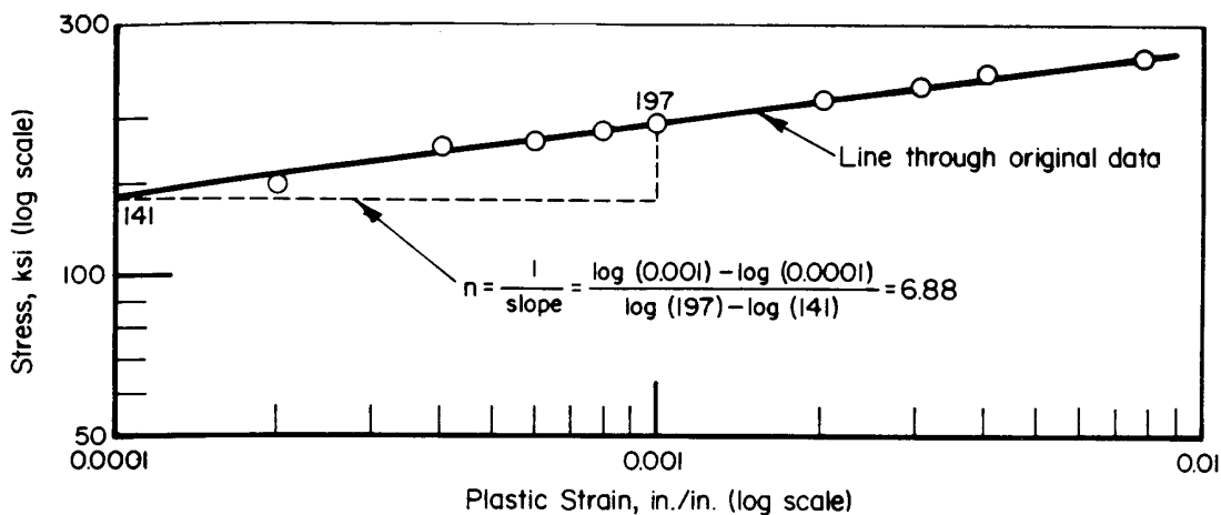
Figure 9.3.2.4. Graphical approximation of Ramberg-Osgood Parameter, n .
