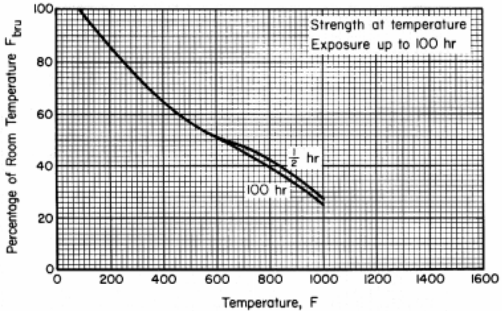
Figure 5.2.1.1.3(a). Effect of temperature on the bearing ultimate strength ( F_{bru} ) of annealed commercially pure titanium.
