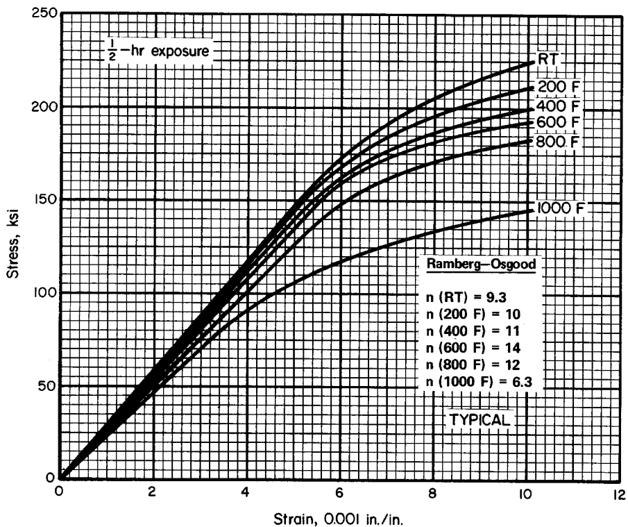
Figure 2.6.7.1.6(b). Typical compressive stress-strain curves at various temperatures for PH15-7Mo (TH1050) stainless steel sheet.
