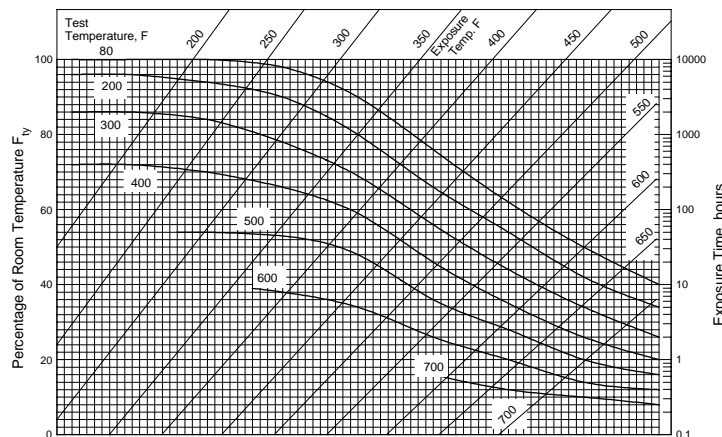
Figure 9.3.1.6.2. Complex-exposure curves.
