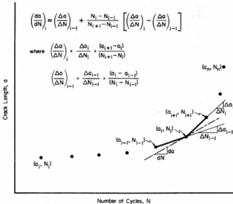
Figure 9.3.5.2. Analytical definition of crack-growth rate calculation.
