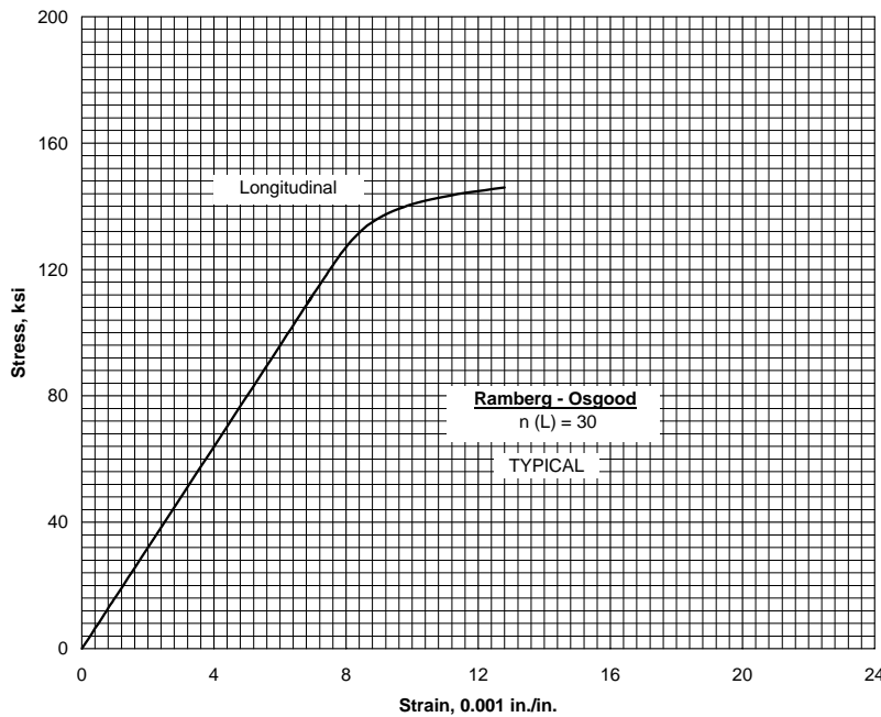
Figure 5.5.2.1.6(b). Typical compressive stress-strain and compressive tangent-modulus curves at room temperature for solution treated and aged ( 1000^\circ\text{F} ) Ti-15V-3Cr-3Sn-3Al alloy sheet.
