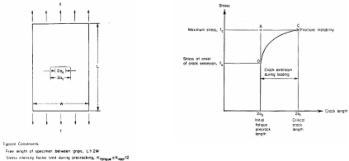
Figure 9.5.1.5.1(a). Middle-tension panel. Figure 9.5.1.5.1(b). Crack growth curve.
