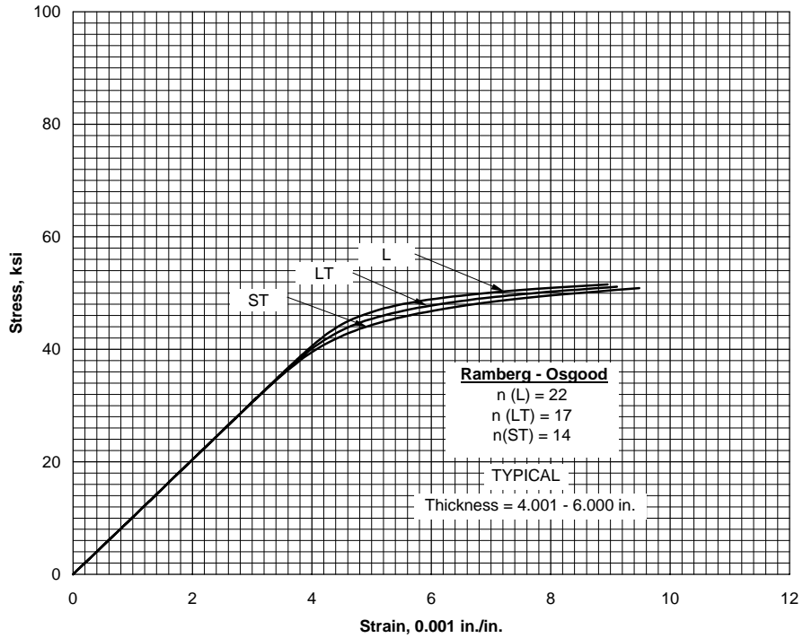
Figure 3.2.7.3.6(a). Typical tensile stress-strain curves for 2219-T852 aluminum alloy hand forging at room temperature.
