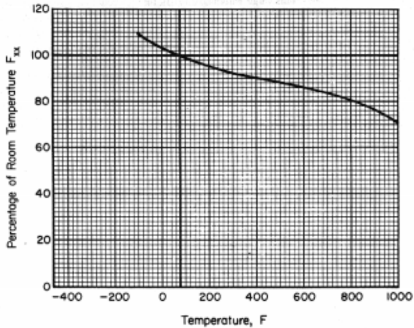
Figure 9.4.2.5.3. Typical effect of temperature presentation.
