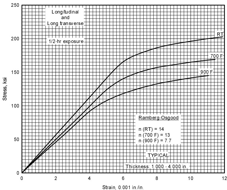
Figure 2.4.2.1.6(a). Typical tensile stress-strain curves for 9Ni-4Co-0.20C steel plate at various temperatures.
