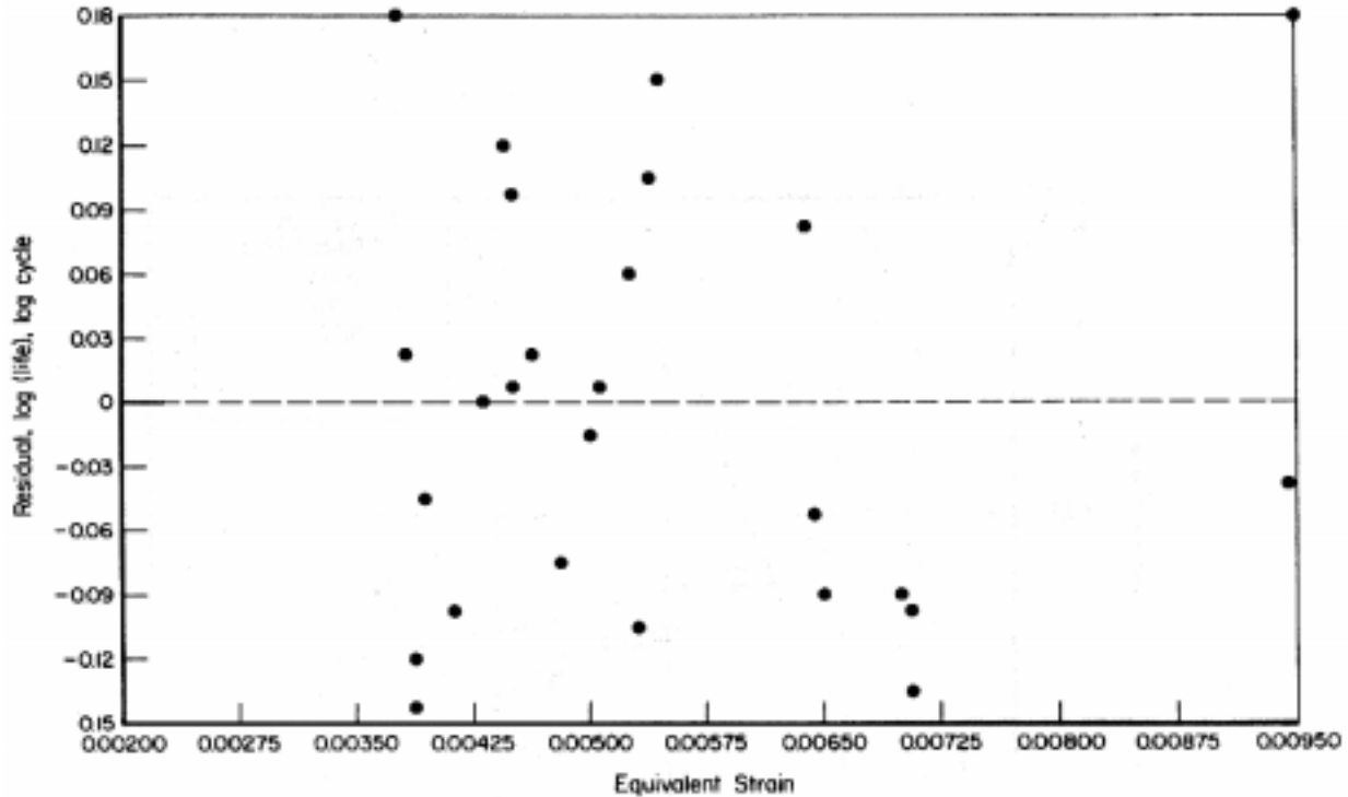
Figure 9.3.4.17(b). Residual plot of fatigue-life model for initial parameter estimates.
