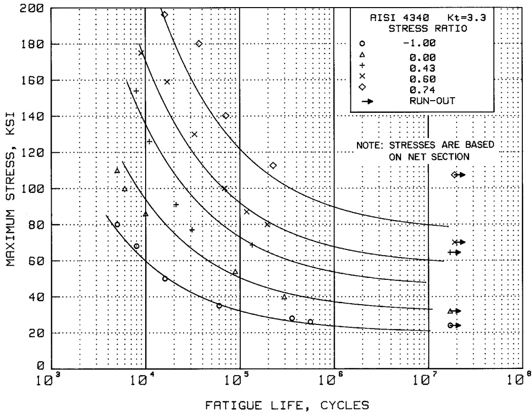
Figure 2.3.1.3.8(l). Best-fit S/N curves for notched, K_t = 3.3 , AISI 4340 alloy steel bar, F_{1u} = 200 ksi, longitudinal direction.
