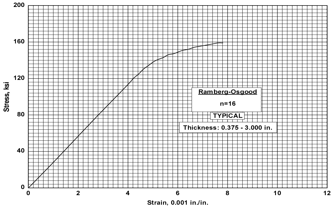
Figure 2.6.8.3.6(a). Typical tensile stress-strain curve for 17-4PH (H1000) stainless steel casting at room temperature.
