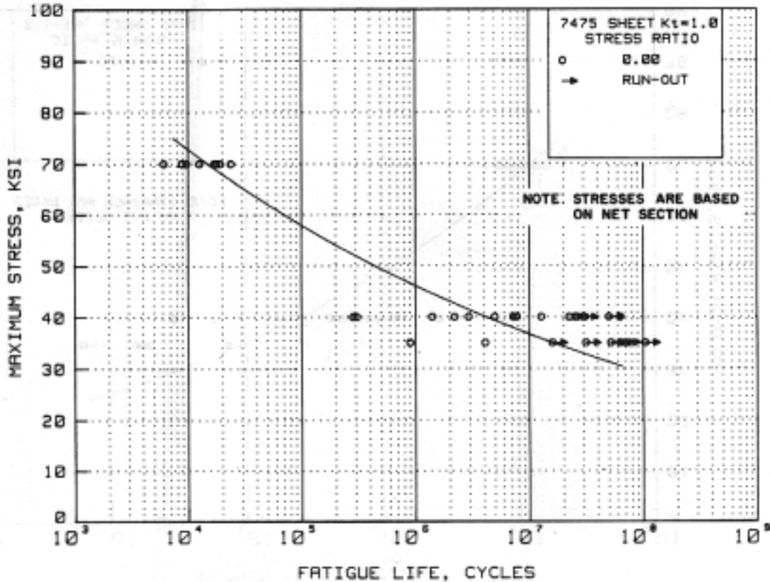
Figure 3.7.8.1.8(b). Best-fit S/N curve for unnotched 7475-T61 and T761 sheet, thickness \leq 0.125 inch, longitudinal and long transverse directions.
