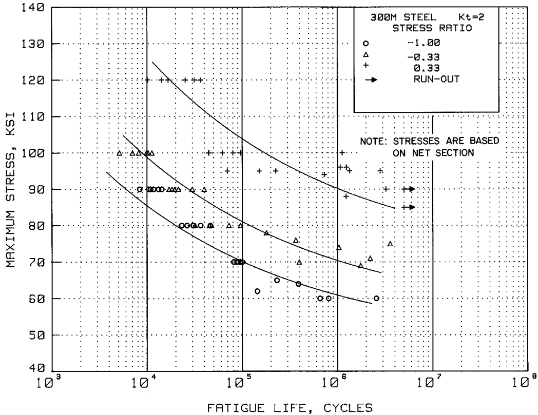
Figure 2.3.1.4.8(b). Best-fit S/N curves for unnotched, K_t = 2.0 , 300M alloy forged billet, F_u = 280 ksi, longitudinal direction.
