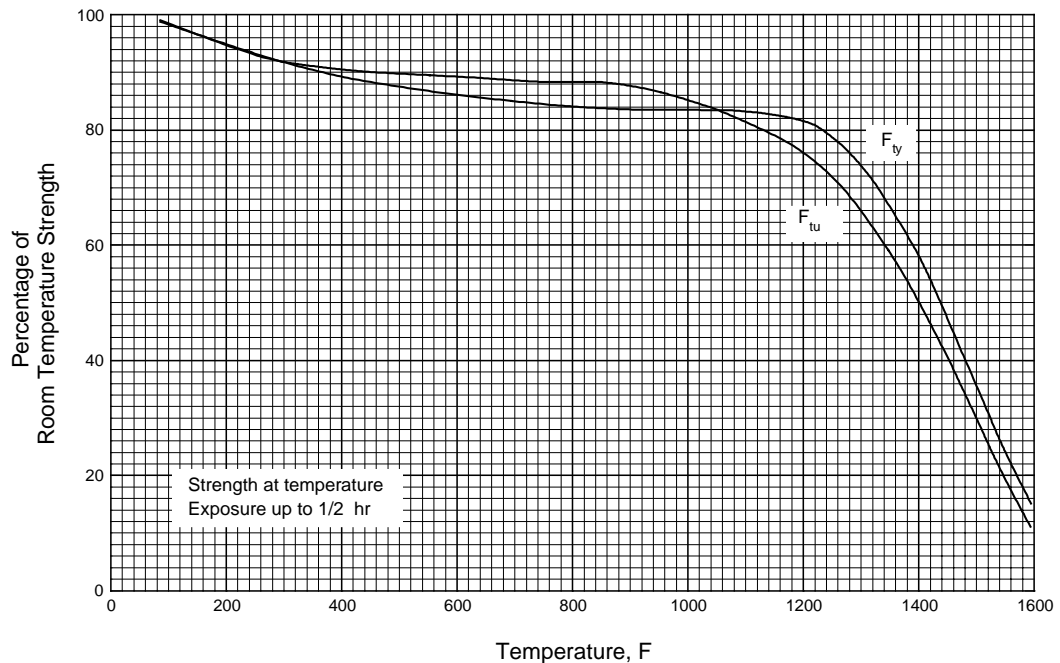
Figure 6.3.4.1.1. Effect of temperature on the tensile ultimate strength (F tu ) and the tensile yield strength (F y ) of solution treated and aged (creep rupture heat treatment) of Inconel 706.
