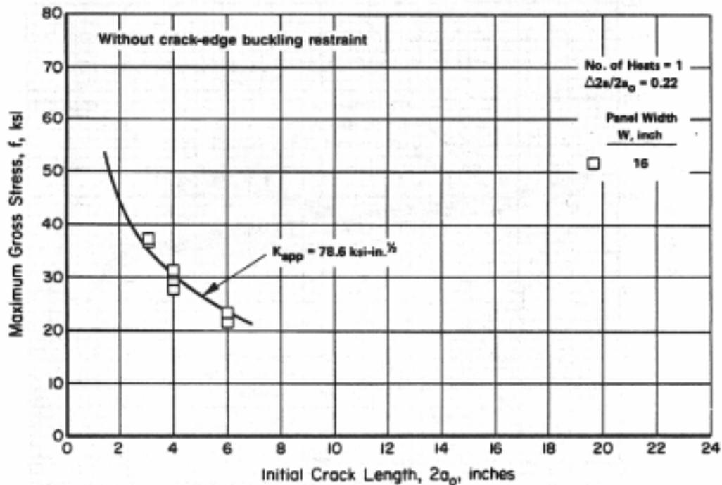
Figure 3.7.8.10(d). Residual strength behavior of 0.063-inch-thick 7475-T61 clad aluminum alloy sheet at room temperature. Crack orientation is T-L. [Reference 3.2.5.1.9(d).]
