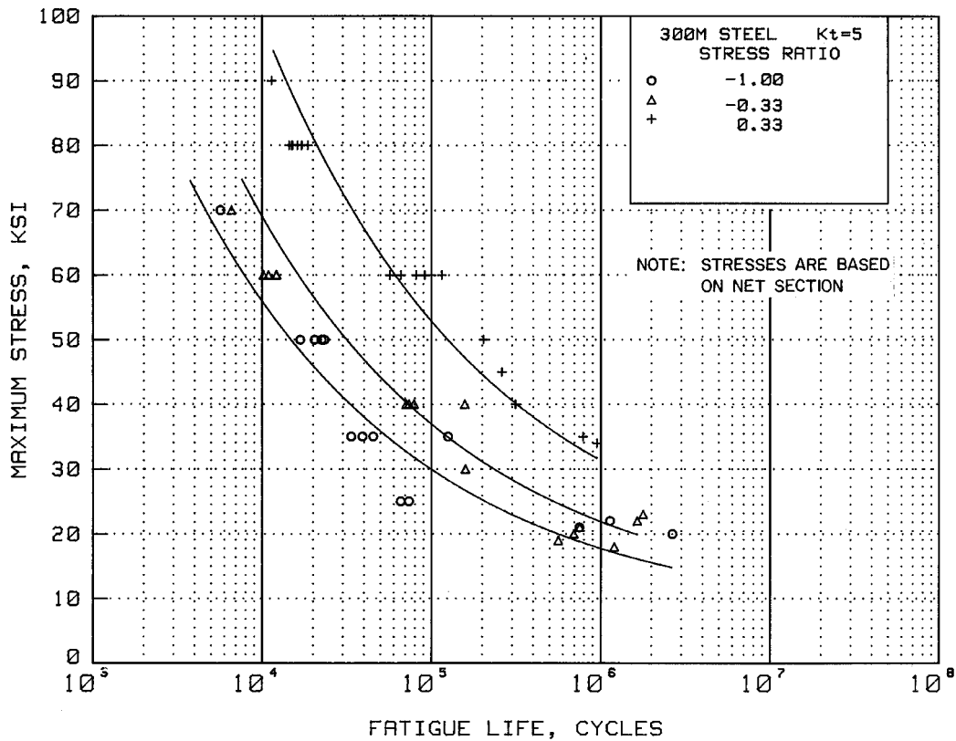
Figure 2.3.1.4.8(d). Best-fit S/N curves for notched, K_t = 5.0 , 300M alloy forged billet, F_{1u} = 280 ksi, longitudinal direction.
