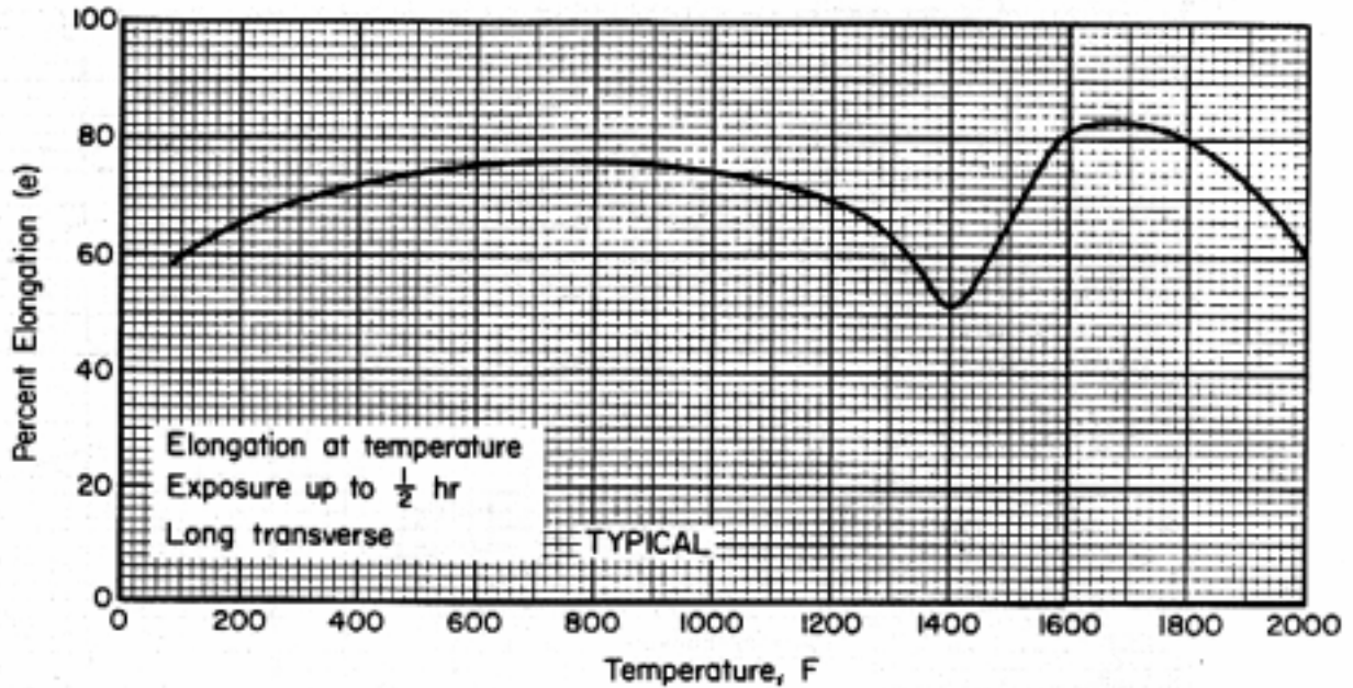
Figure 6.4.2.1.5. Effect of temperature on elongation (e) of HS 188 sheet.
