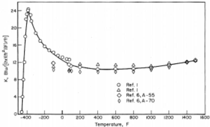
FIGURE 9.3.1.4(a). Typical working curve for thermal conductivity.
