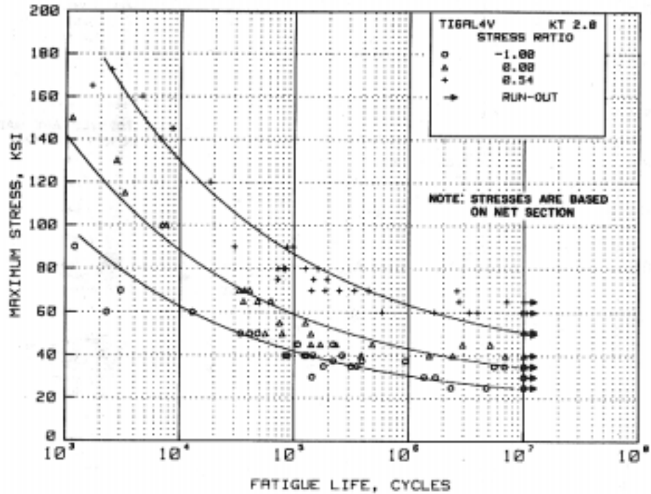
Figure 5.4.1.2.8(b). Best-fit S/N curves for notched, K_t = 2.8 , solution-treated and aged Ti-6Al-4V sheet at room temperature, longitudinal direction.
