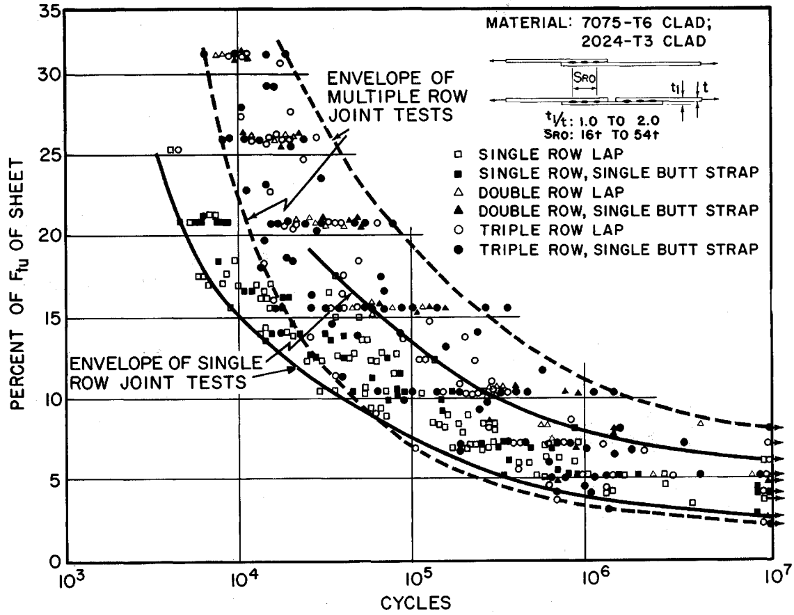
Figure 8.2.3.2.2(a). Fatigue strength of spot-welded joints in aluminum alloy sheet. Load Ratio = 0.05 (static failure by tearing sheet).
