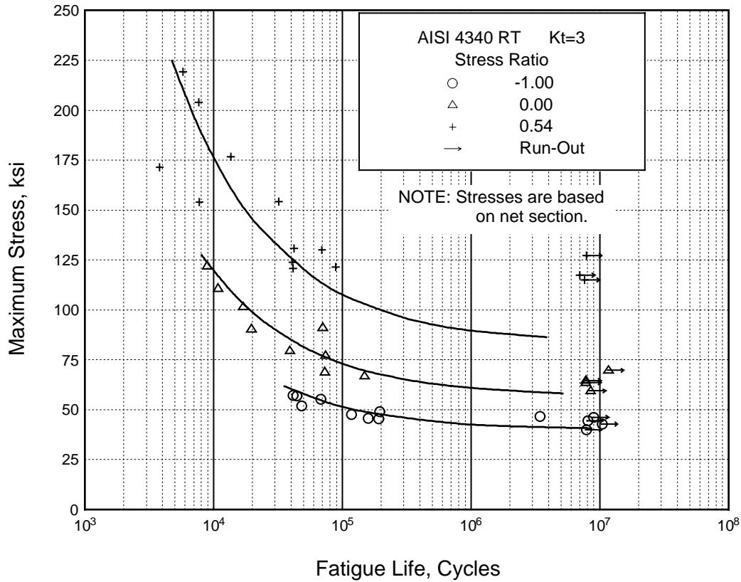
Figure 2.3.1.3.8(o). Best-fit S/N curves for notched, K_t = 3.0 , AISI 4340 alloy steel bar, F_u = 260 ksi, longitudinal direction.
