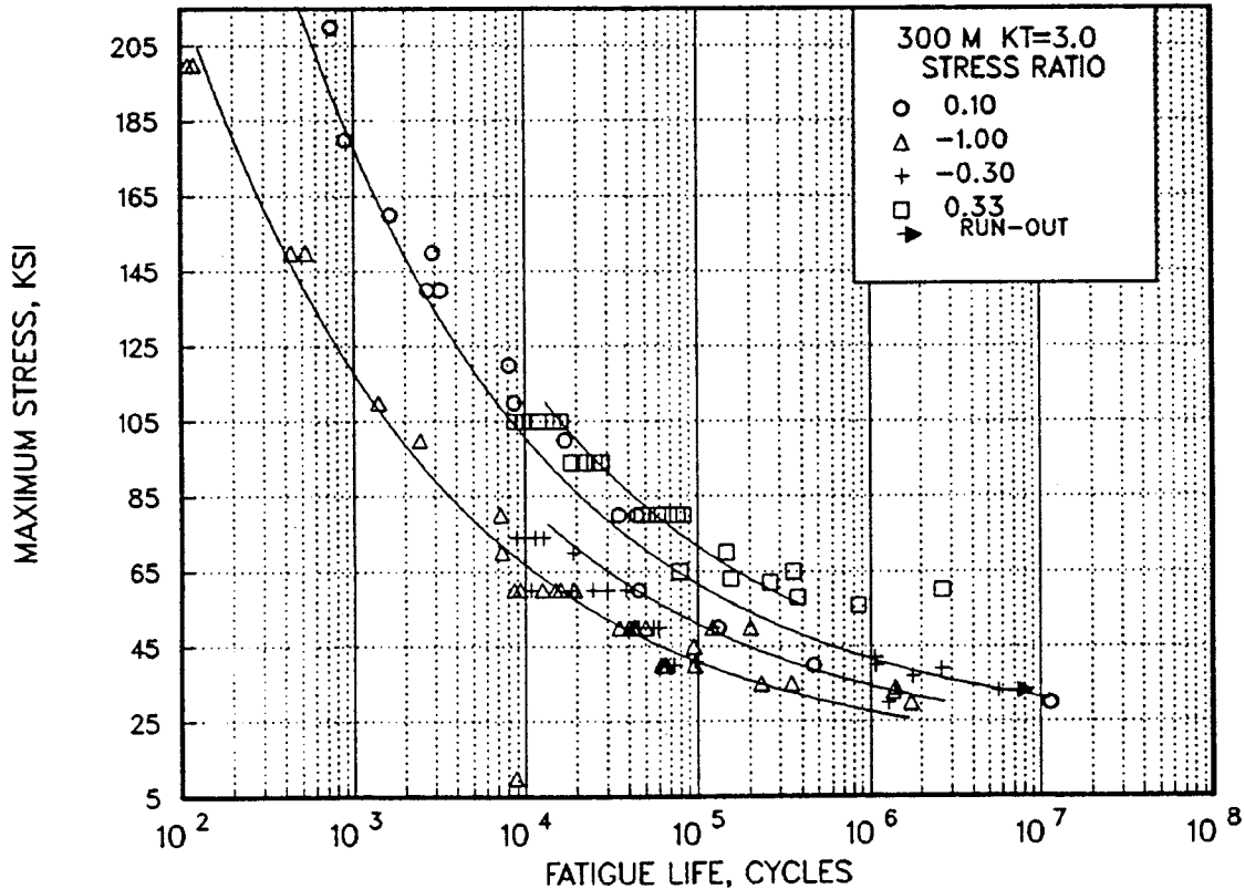
Figure 2.3.1.4.8(c). Best-fit S/N curves for notched, K_t = 3.0 , 300M alloy forging, F_{1u} = 280 ksi, longitudinal and transverse directions.
