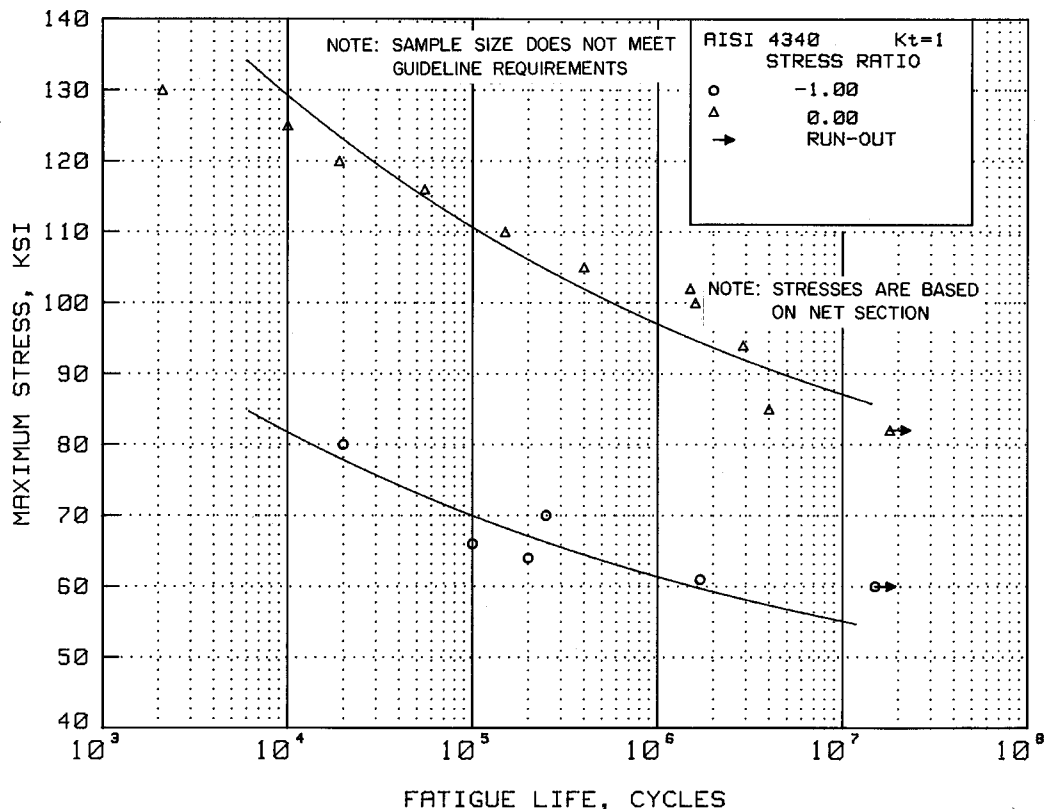
Figure 2.3.1.3.8(g). Best-fit S/N curves for unnotched AISI 4340 alloy steel bar at 800°F, F_u = 150 ksi, longitudinal direction.
