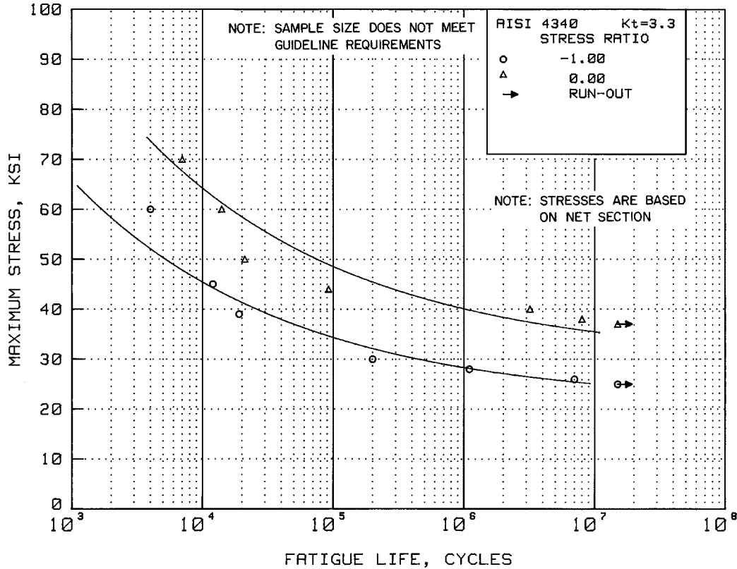
Figure 2.3.1.3.8(j). Best-fit S/N curves for notched, K_t = 3.3 , AISI 4340 alloy steel bar at 1000^\circ\text{F} , F_{10} = 150 ksi, longitudinal direction.
