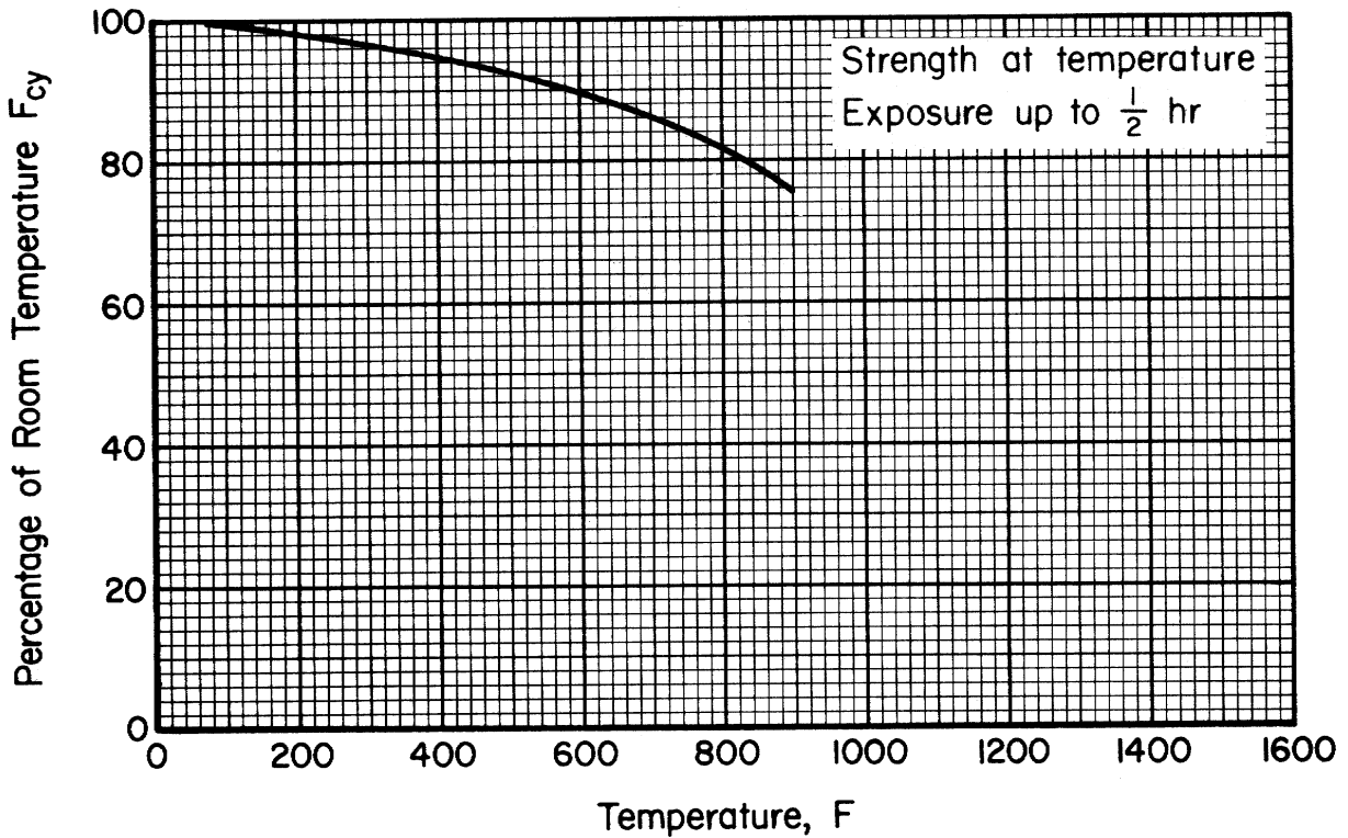
Figure 2.6.6.3.2. Effect of temperature on the compressive yield strength ( F_{cy} ) of 15-5PH (H1150) stainless steel bar.
