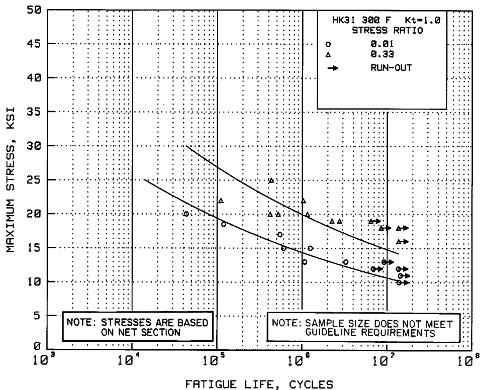
Figure 4.2.3.2.8(b). Best-fit S/N curves for notched, K_t = 2.4 , ZK60A-T5 extruded bar, longitudinal direction.
